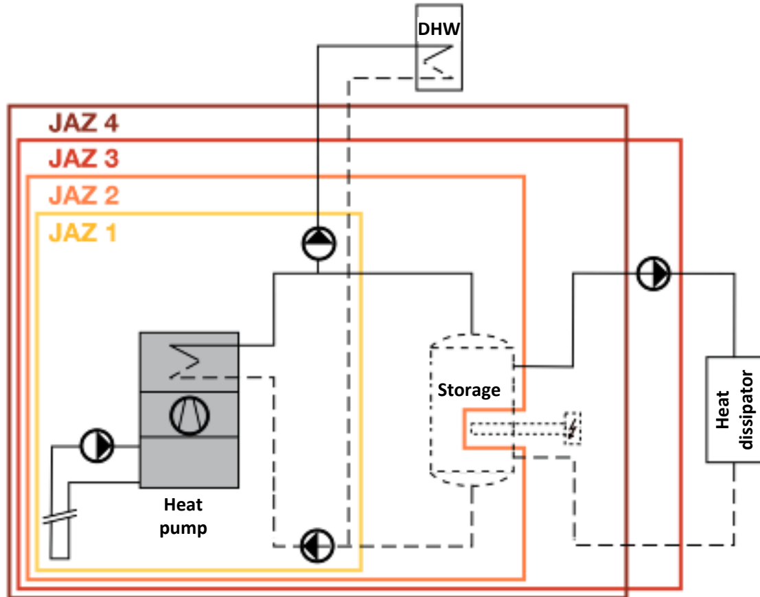
Fig. 2. System boundaries of different definitions for the annual efficiency of heat pumps
