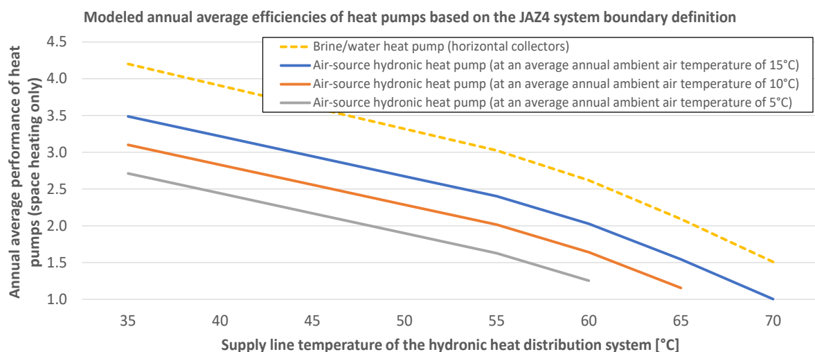
Fig. 3. Implemented annual efficiencies of heat pumps
